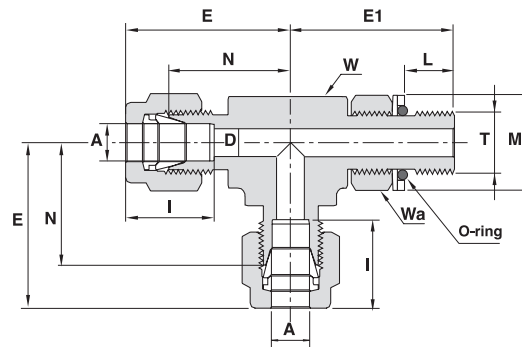
TUBE (METRIC) TO ISO PARALLEL THREAD (POSITIONABLE)*
