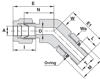
TUBE (METRIC) TO ISO PARALLEL THREAD (POSITIONABLE)*
