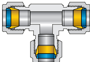
UNION TEE - 764 L
