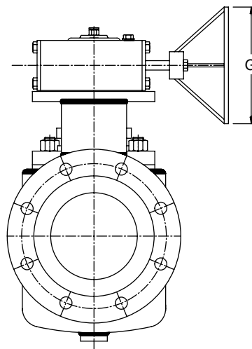
ZFR 03R - Full with Gear
