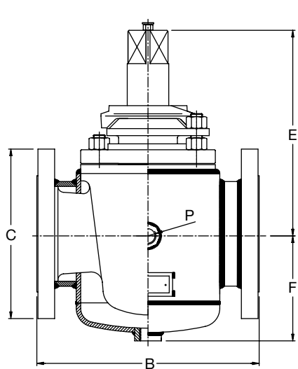
ZFC 03R - Full with Wrench
