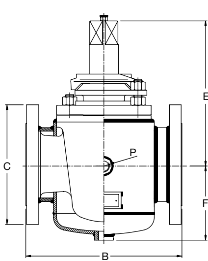
ZRC 03R - Regular with Wrench
